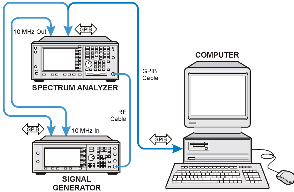
Figure 3 Connecting the GPIB Interface (Signal Studio for Enhanced Multitone and Pulse Building only )
