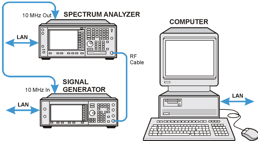
Figure 17 Connecting the LAN Interface to an Existing Network (Signal Studio for Enhanced Multitone and Pulse Building only )
